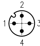
Contact arrangement
